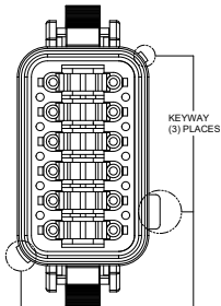
P/N AT06-12SC KEY-C CONFIGURATION STANDARD COLOR: GREEN
