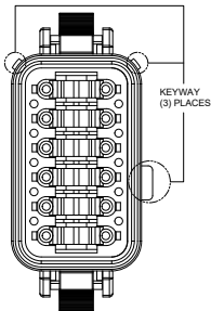
P/N AT06-12SB KEY-B CONFIGURATION STANDARD COLOR: BLACK
