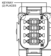
P/N AT04-08PB KEY-B CONFIGURATION STANDARD COLOR: BLACK
